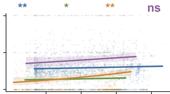
Selfing mating system
