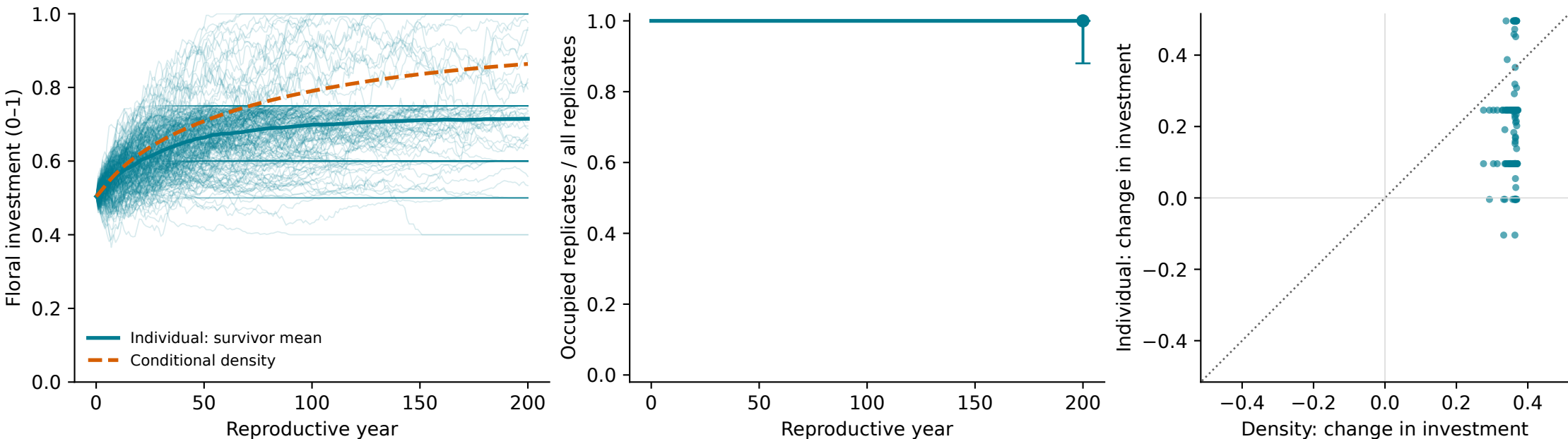
recovery_resident_immigrants_uninterrupted | production | 128 independent histories, 256/256 occupied at endpoint
