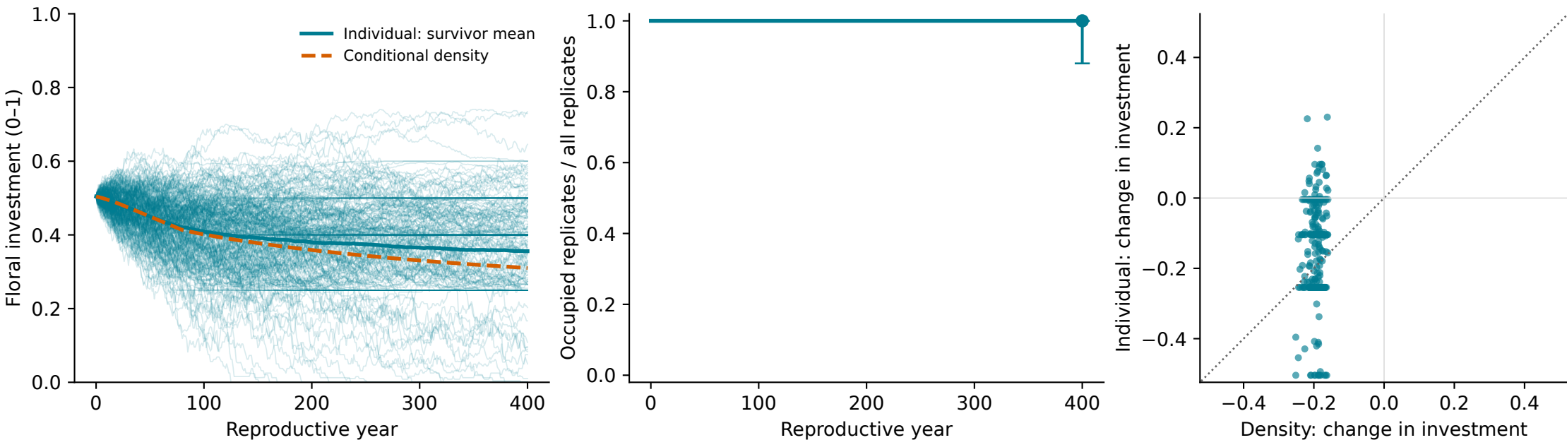
life_perennial10_lifetime | production | 128 independent histories, 256/256 occupied at endpoint
