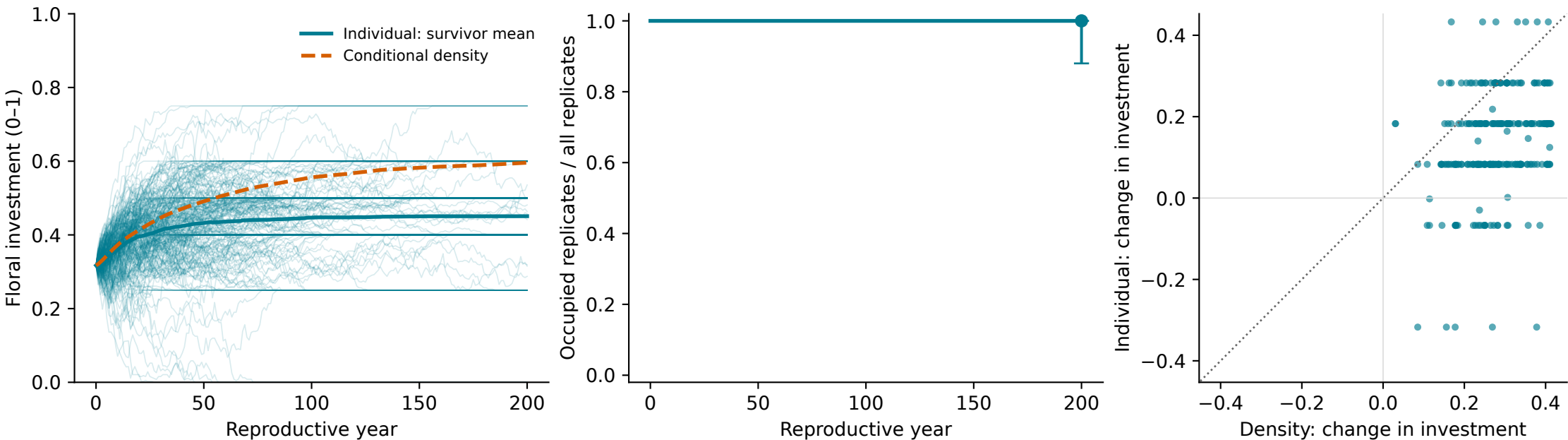
transport_d0_s3 | heldout | 128 independent histories, 256/256 occupied at endpoint
