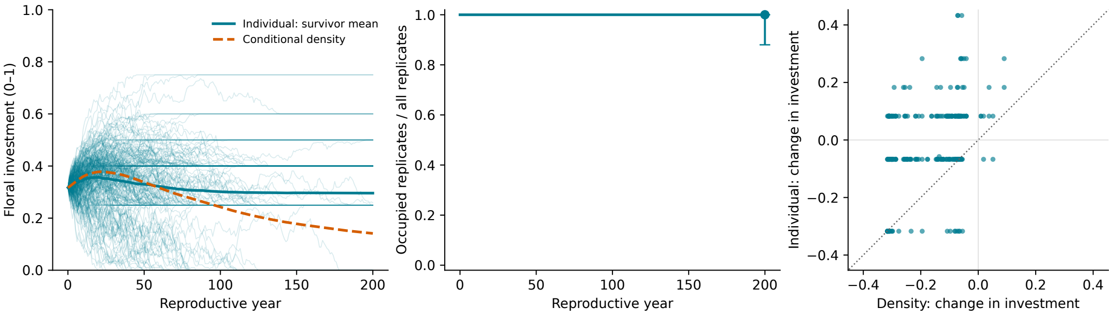
transport_d3_s3 | heldout | 128 independent histories, 256/256 occupied at endpoint
