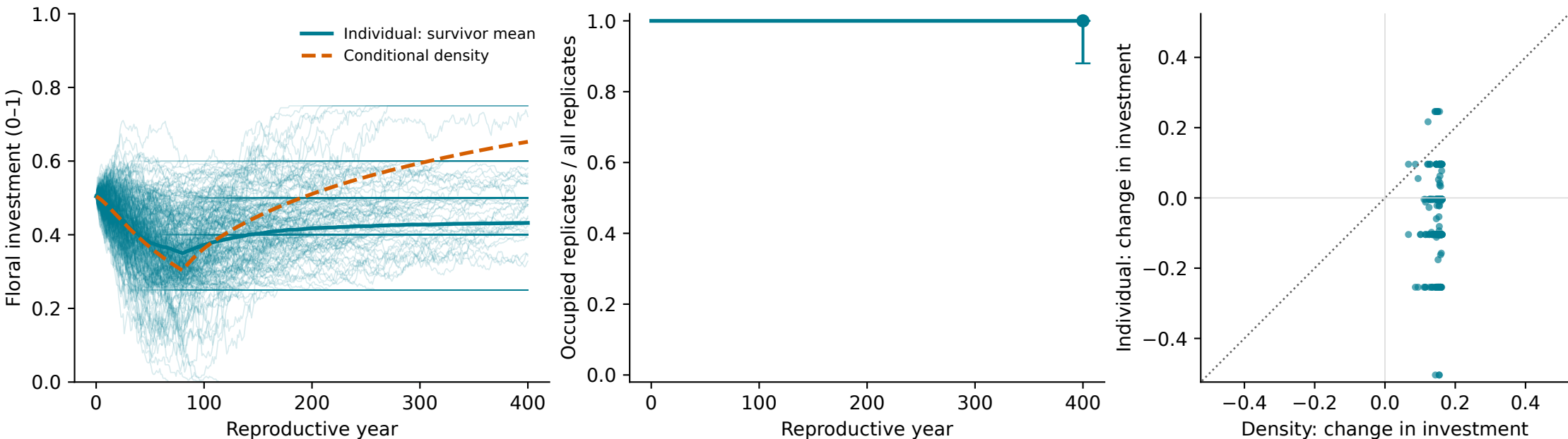
life_perennial4_annual | production | 128 independent histories, 256/256 occupied at endpoint
