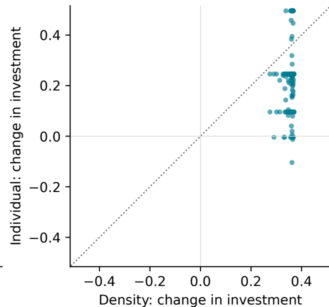
recovery_source_immigrants_uninterrupted | production | 128 independent histories, 256/256 occupied at endpoint
