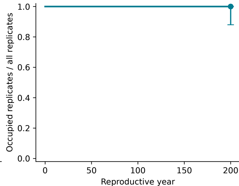
recovery_source_immigrants_uninterrupted | production | 128 independent histories, 256/256 occupied at endpoint
