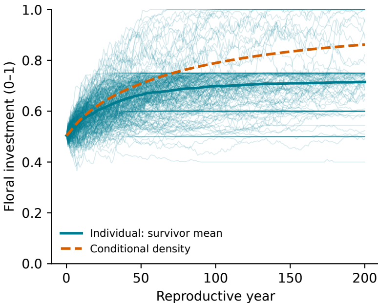
recovery_source_immigrants_uninterrupted | production | 128 independent histories, 256/256 occupied at endpoint
