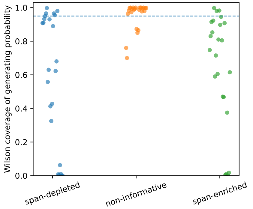
B. Interval coverage
