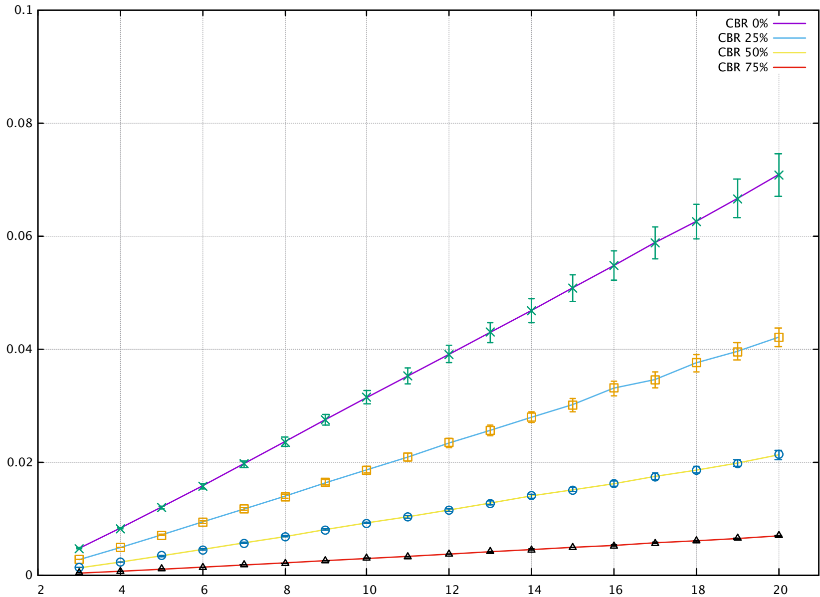
Burtiness vs Arrival delay of On/Off source sharing resources with CBR
