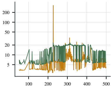
rod-twist
