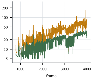
rod-twist
