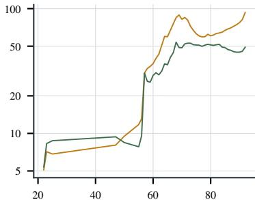
puffer-ball
