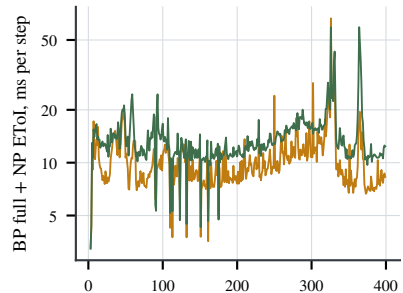
n-body
