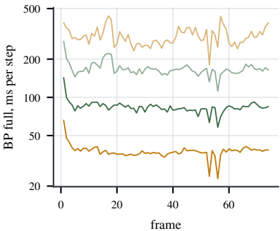
n-body
