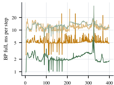
n-body
