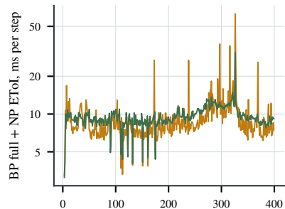
n-body
