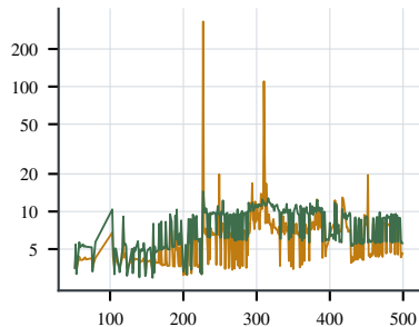
rod-twist
