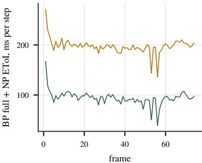
n-body
