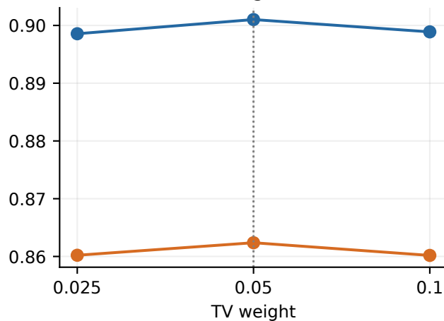
Slice-averaged SSIM ↑
