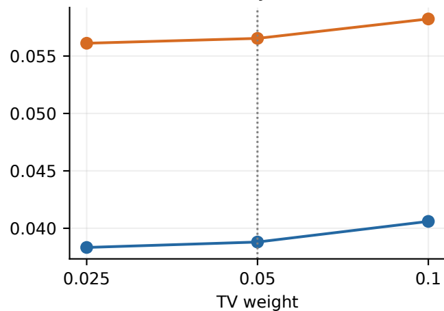
Boundary MAE ↓
