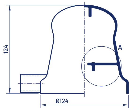
FIG. 1 HALF SECTION · 1:2.5
