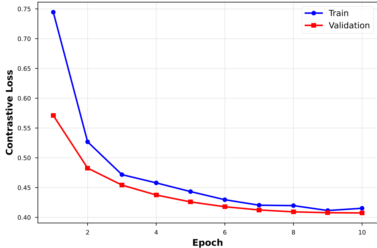
(b) Fusion Module Training
