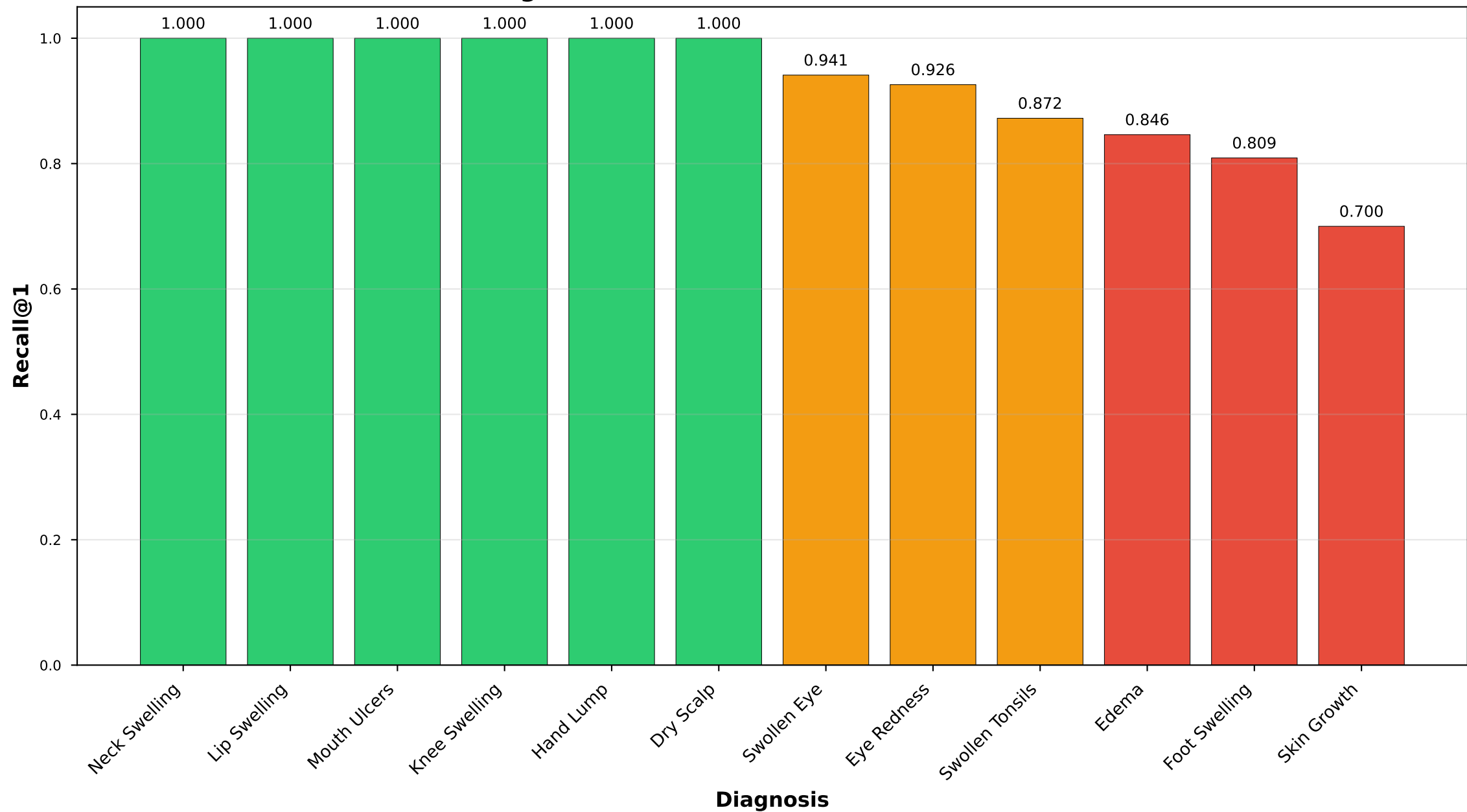
Per-Diagnosis Retrieval Performance (Fusion Mode)
