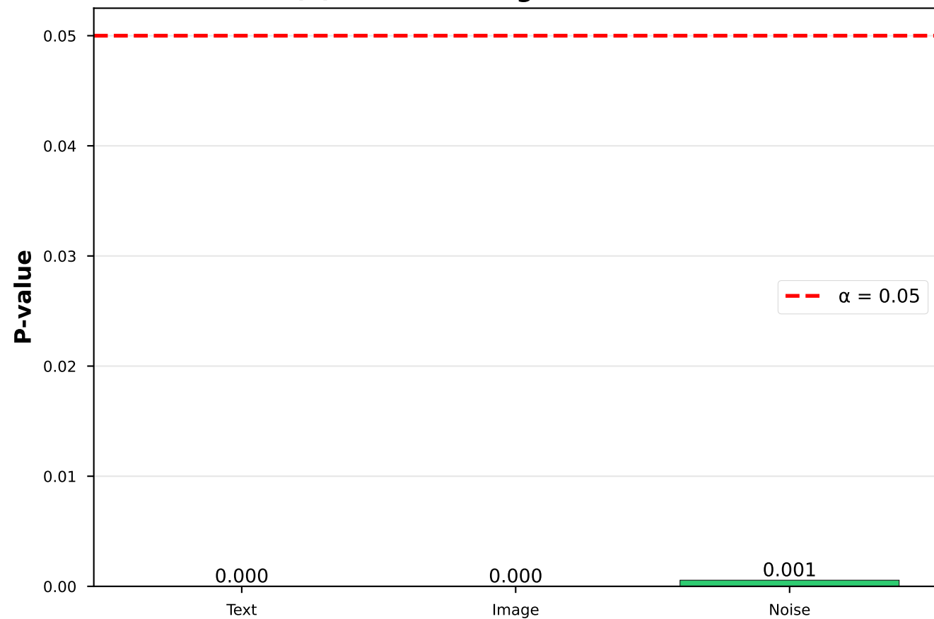
(a) Statistical Significance Tests
