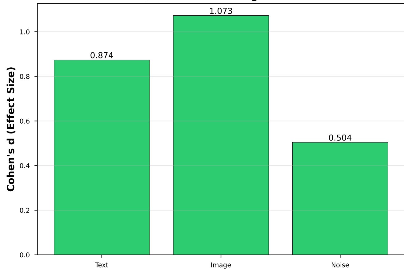
(b) Effect Size Magnitude
