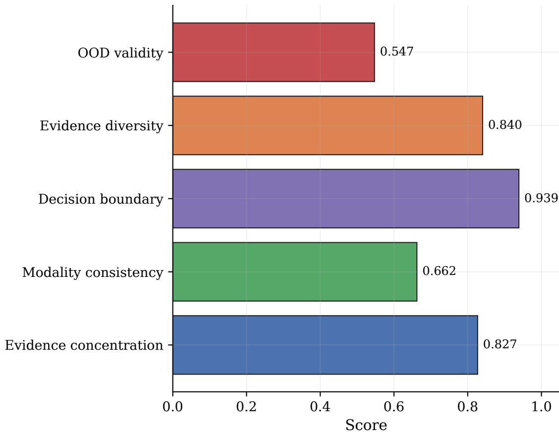
Constraint mean scores
