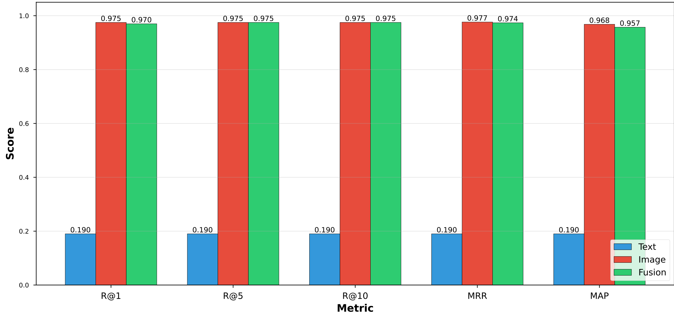
Retrieval Performance: Modality Comparison
