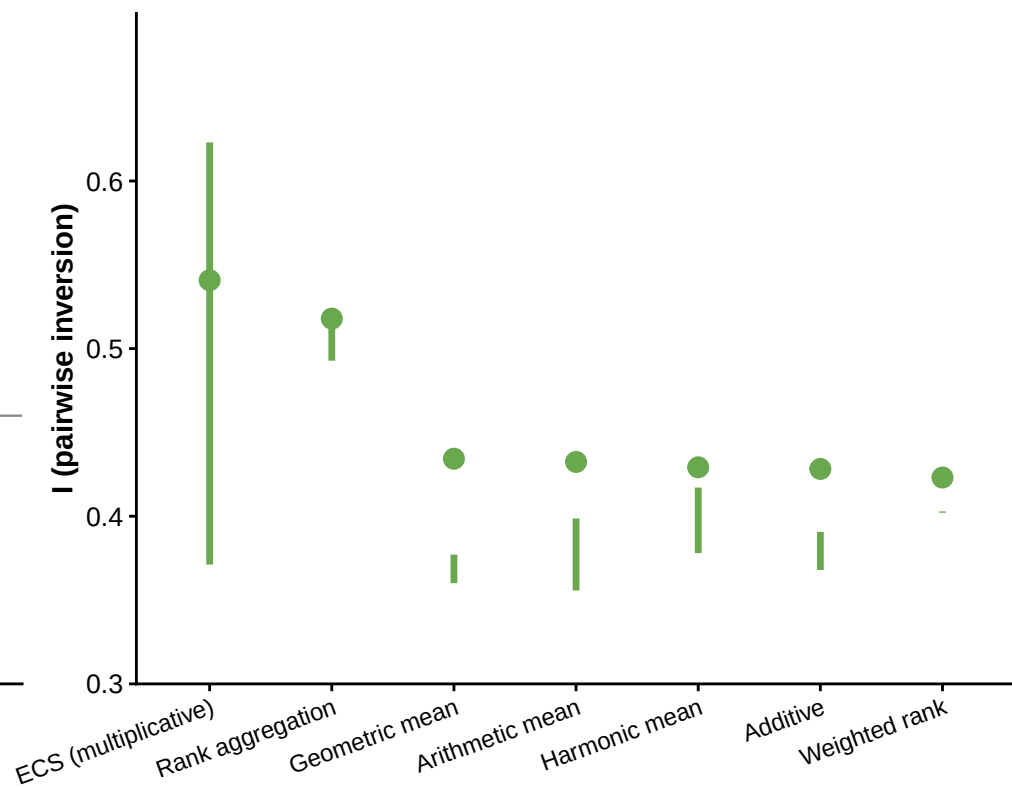
b | Pairwise-inversion I (coverage range)
