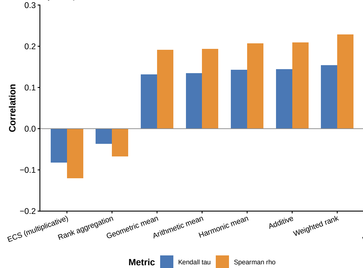
a | Composite rank correlation
