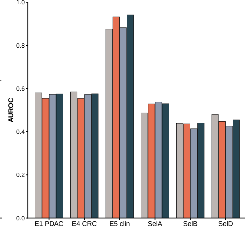
c Alternative missingness conditions (frozen harmonic family)
