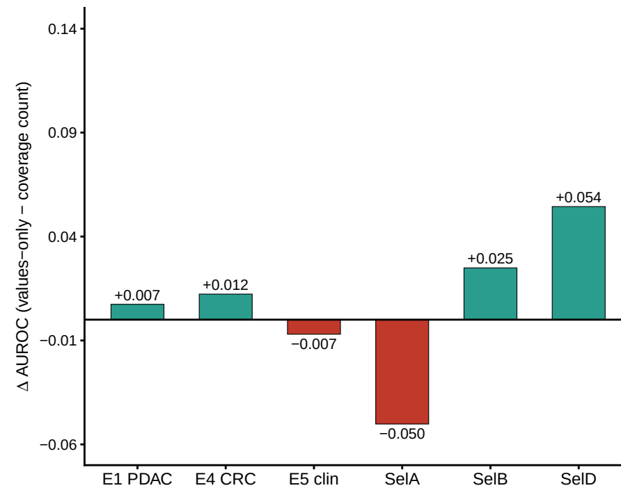
e Delta under matched condition 2: actual values vs coverage only
