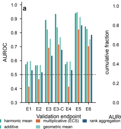
Fixed functional forms
