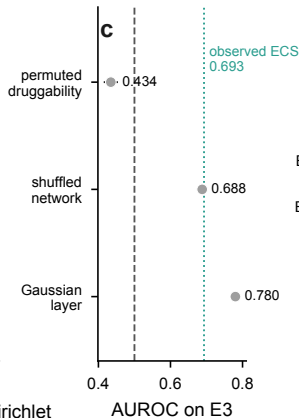
Negative controls
