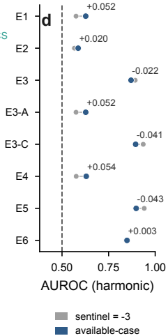
Sentinel-coded vs available-case
