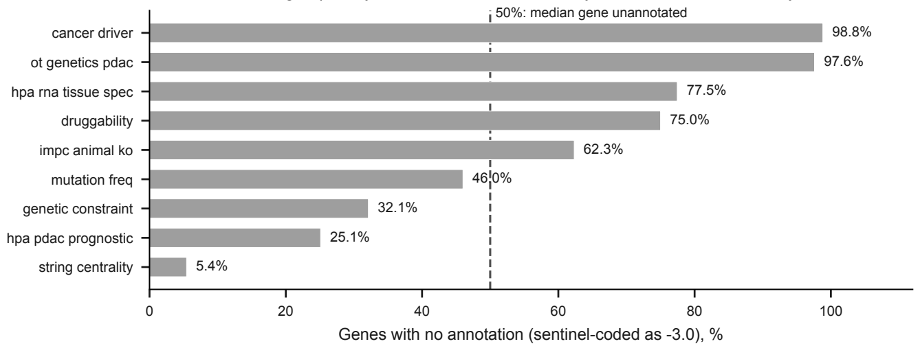
Extended Data Fig. 1 | Study-bias and annotation-density audit of network centrality
