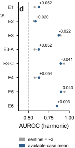
Sentinel-coded versus missingness-aware
