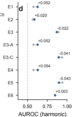
Sentinel-coded versus missingness-aware
