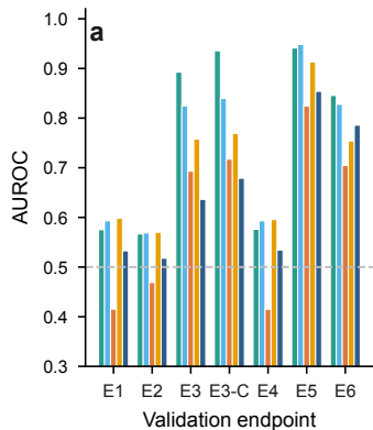
Fixed functional forms
