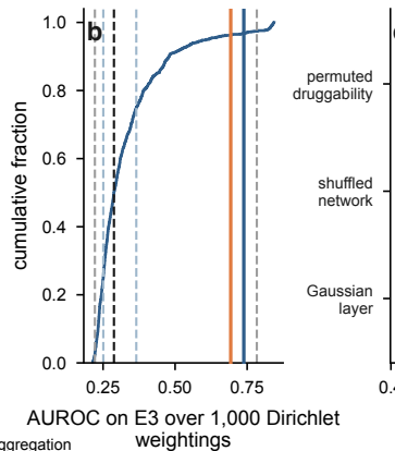
Driver-layer weight space
