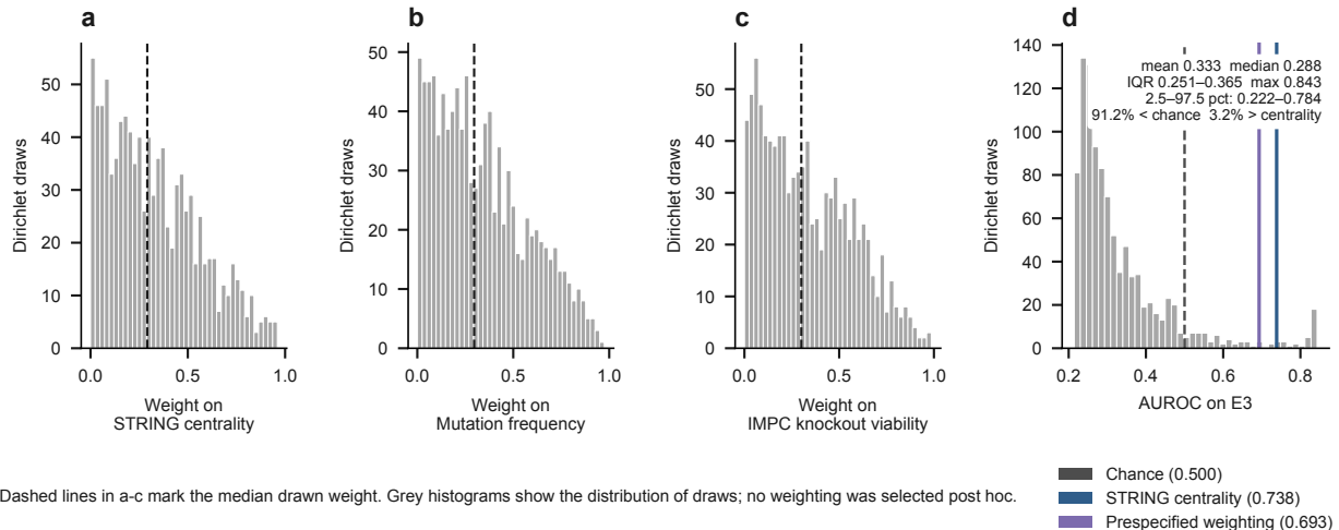
Extended Data Fig. 3 | Full Dirichlet weight-space distribution
