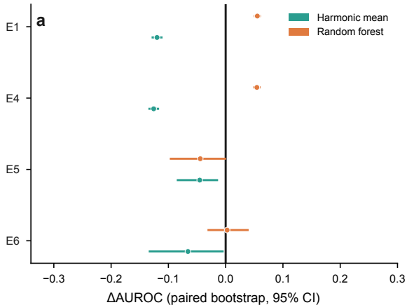
AUROC difference from network centrality
