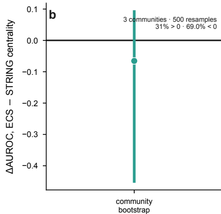
Network-community resampling
