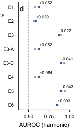
Sentinel-coded versus missingness-aware
