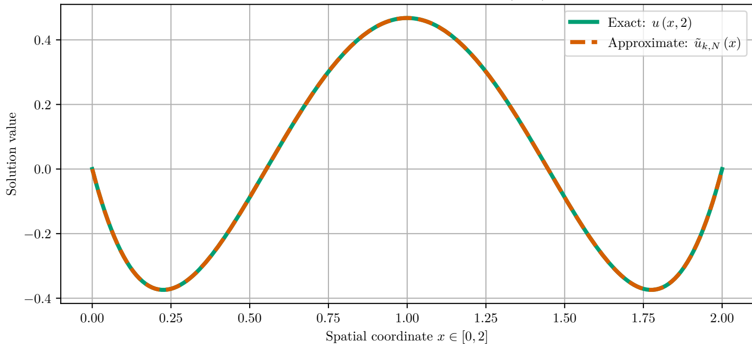
Exact vs Approximate Solution: u(x, t_2)
