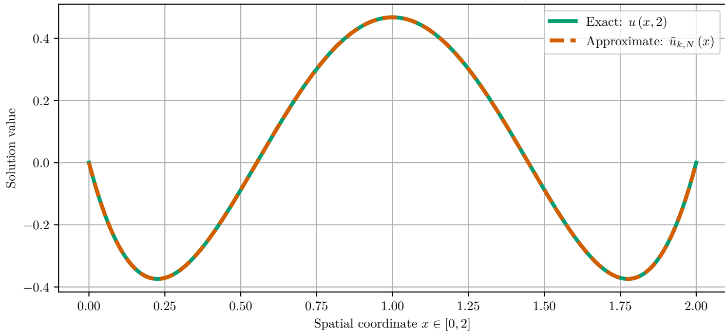
Exact vs Approximate Solution: u(x, t_{10})
