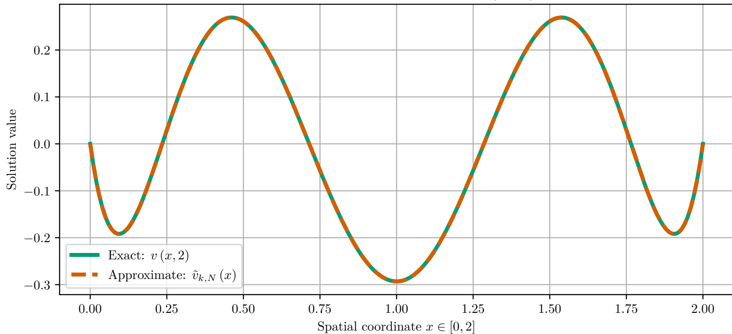
Exact vs Approximate Solution: v(x, t_{10})
