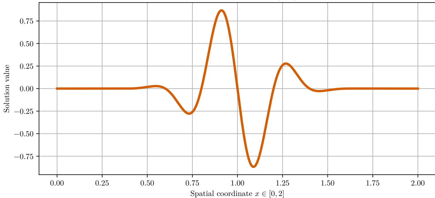
Approximate Solution: v(x, 0)
