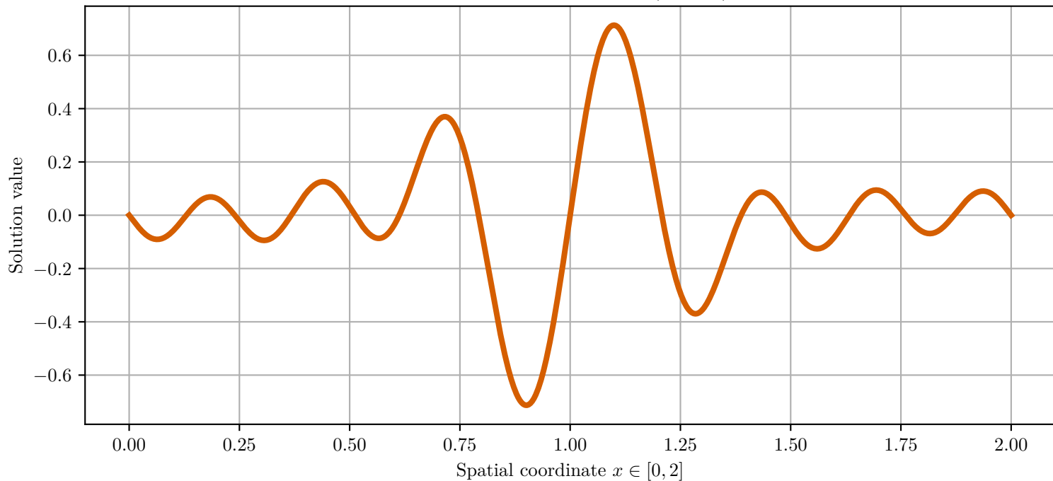
Approximate Solution: u(x, 0.75)
