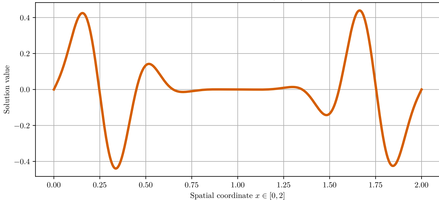
Approximate Solution: v(x, 0.75)
