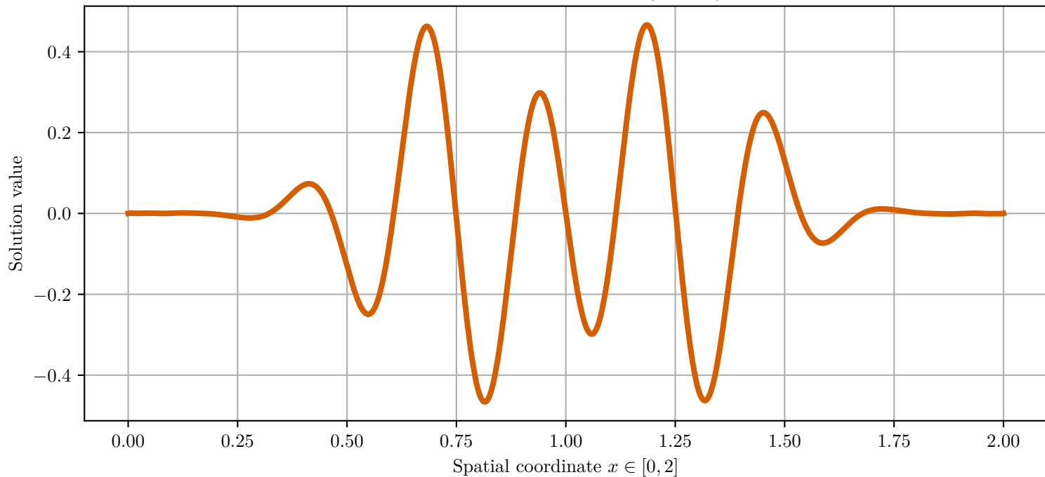
Approximate Solution: v(x, 0.25)
