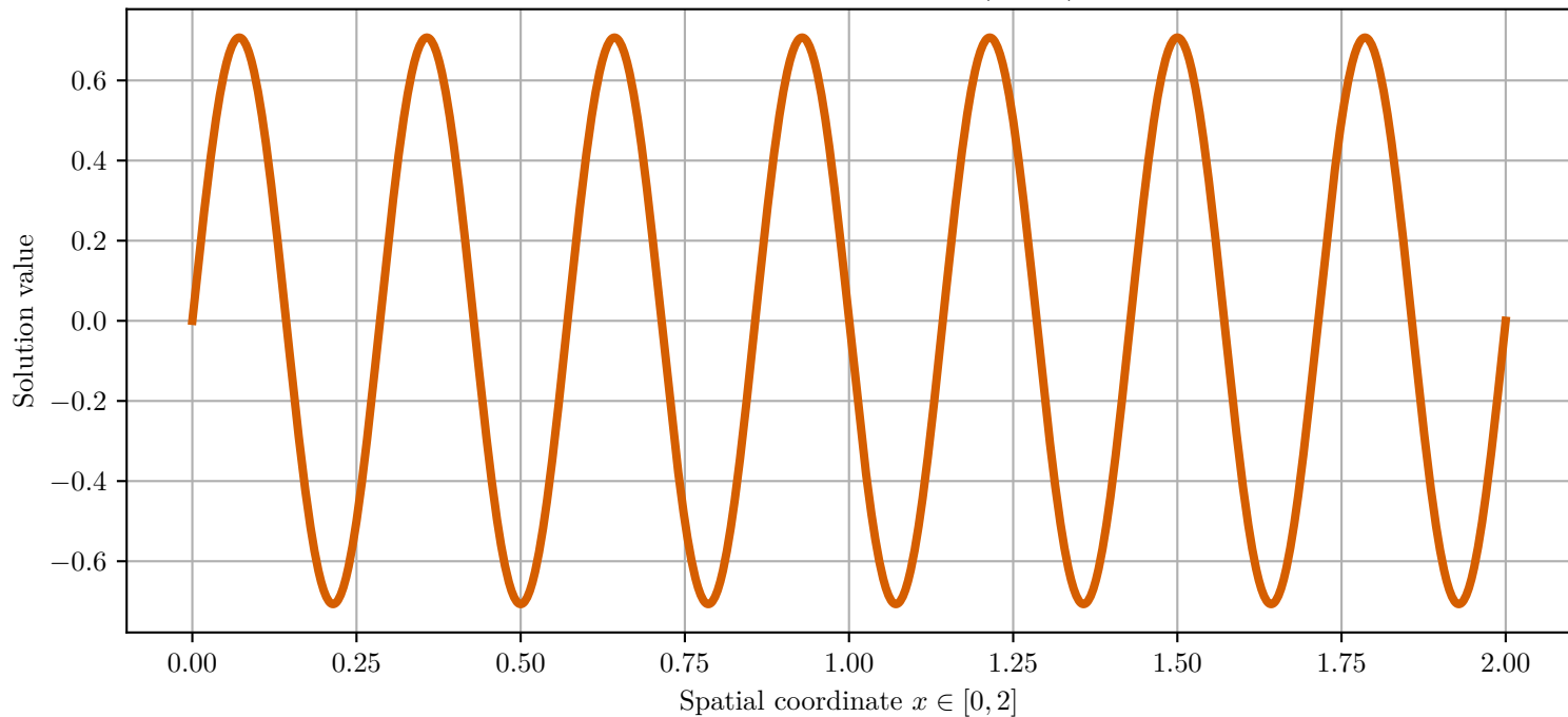
Approximate Solution: u(x, 0.5)
