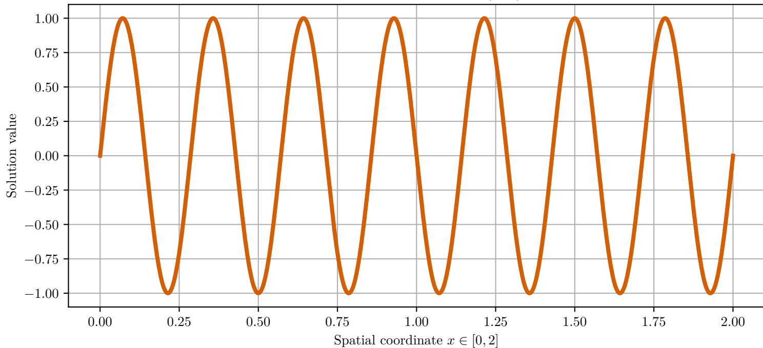
Approximate Solution: u(x, 1)
