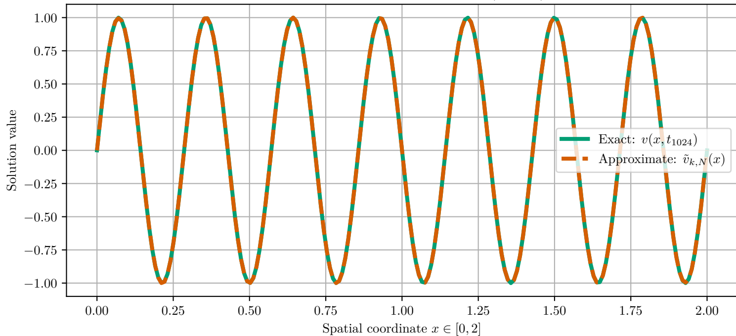
Exact vs Approximate Solution: v(x, t_{1024})
