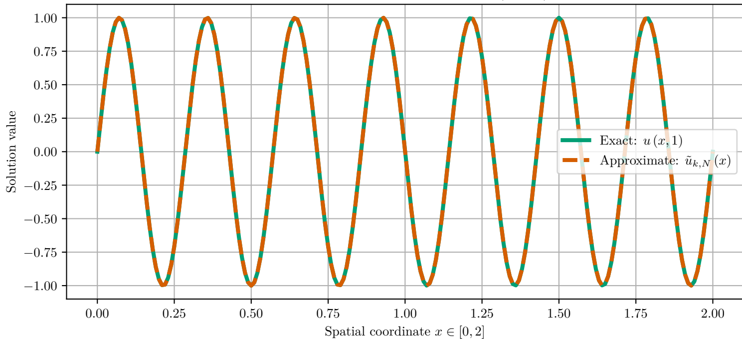
Exact vs Approximate Solution: u(x, t_{256})
