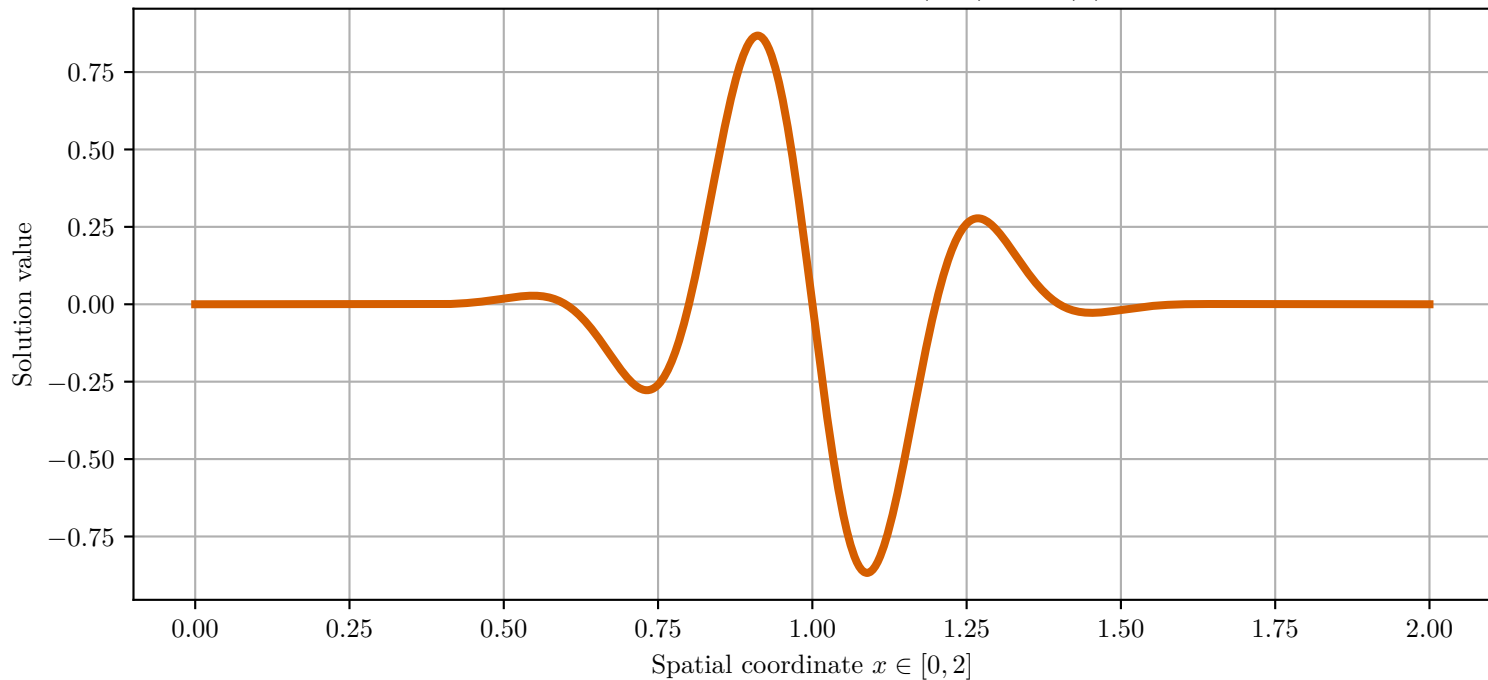
Initial Condition Function: u(x, 0) = \varphi_0(x)
