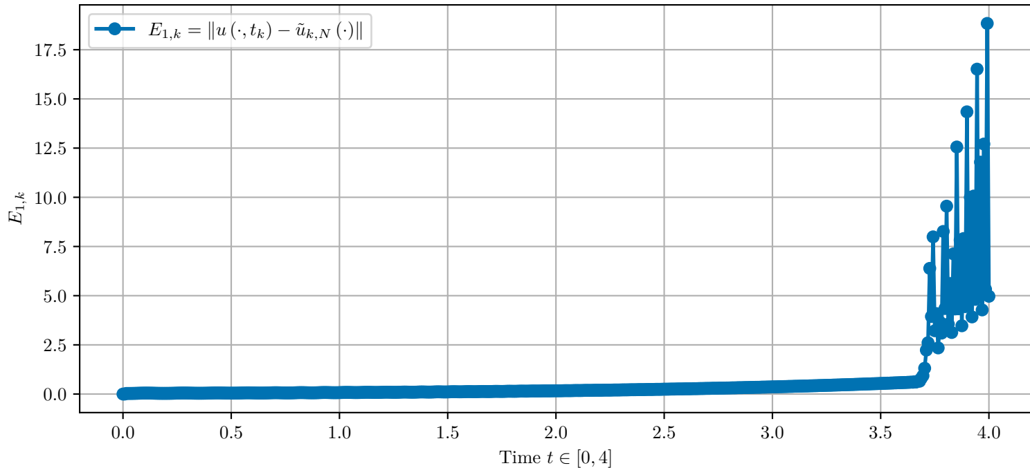
L^2 Error Evolution for u(x, t)
