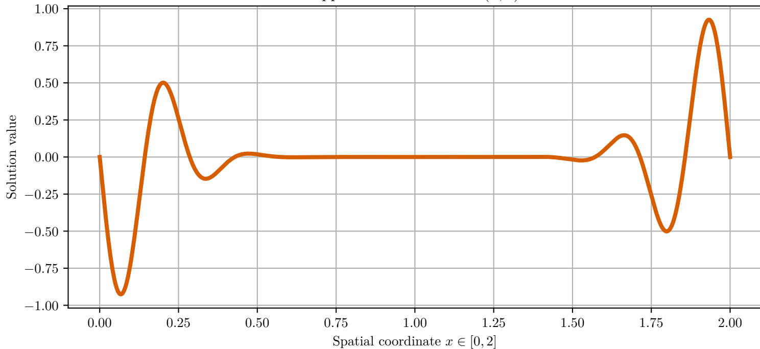
Approximate Solution: v(x, 1)
