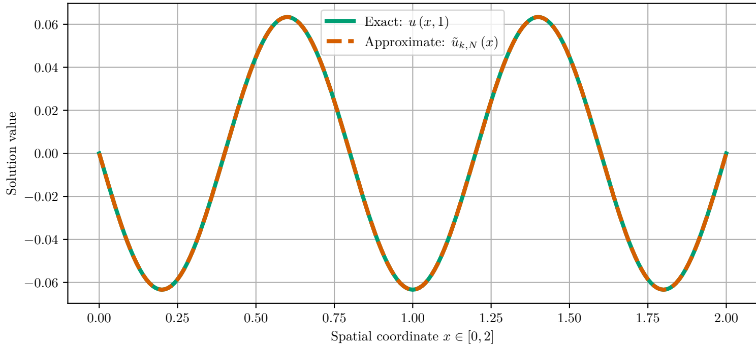
Exact vs Approximate Solution: u(x, t_{2048})
