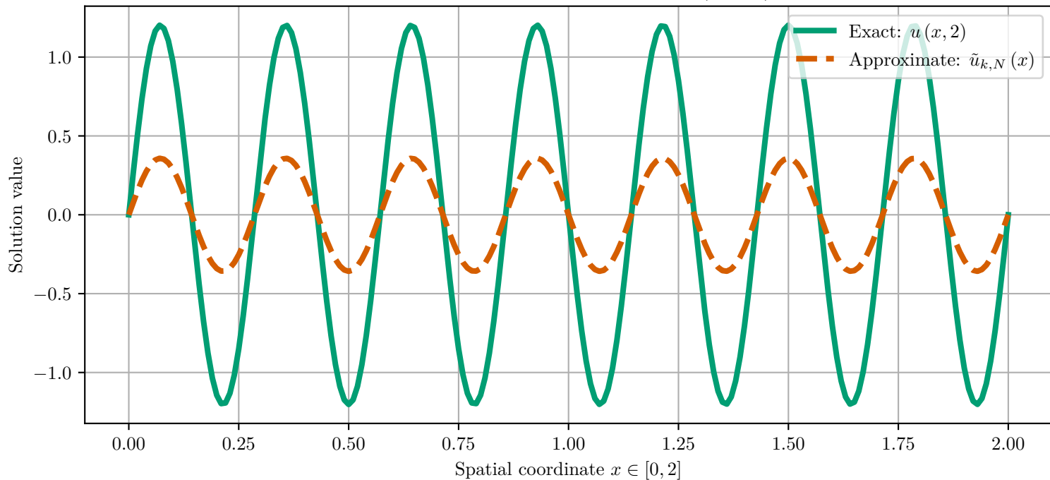
Exact vs Approximate Solution: u(x, t_{512})
