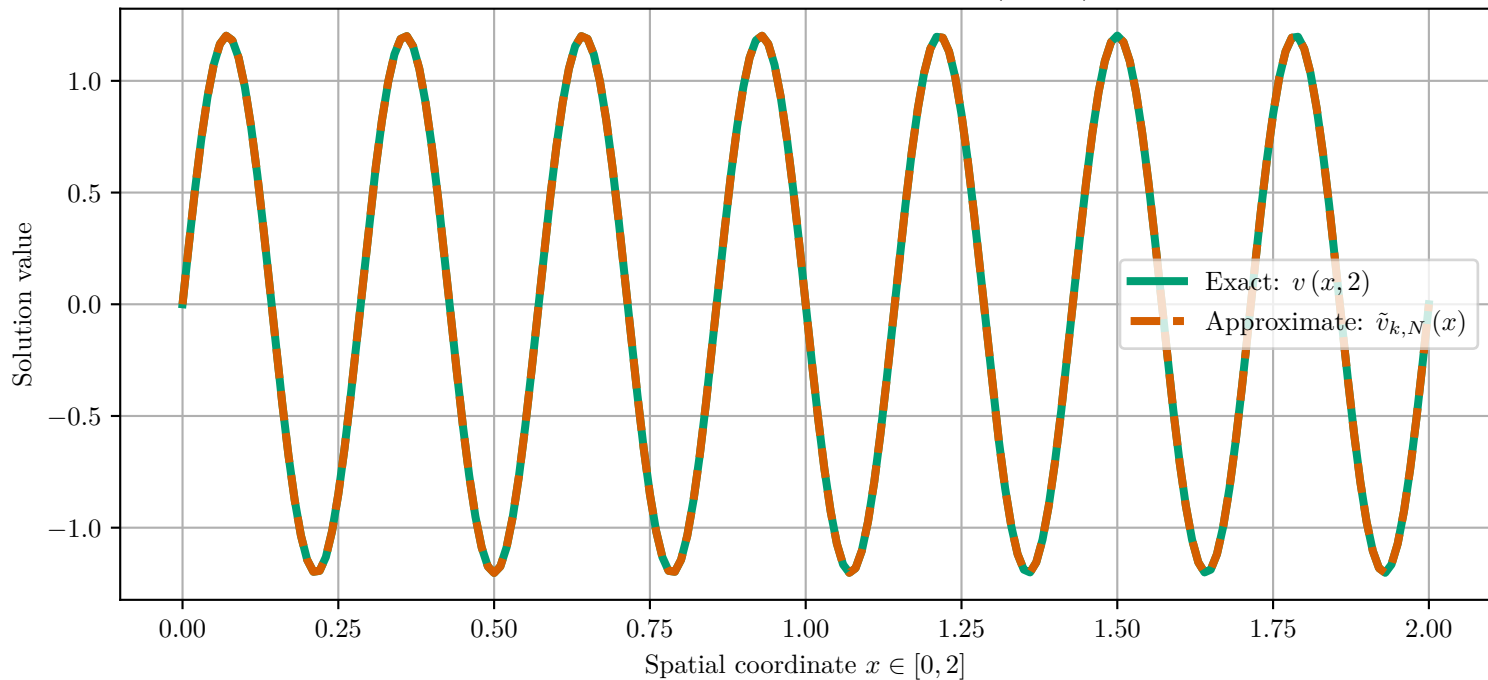
Exact vs Approximate Solution: v(x, t_{512})
