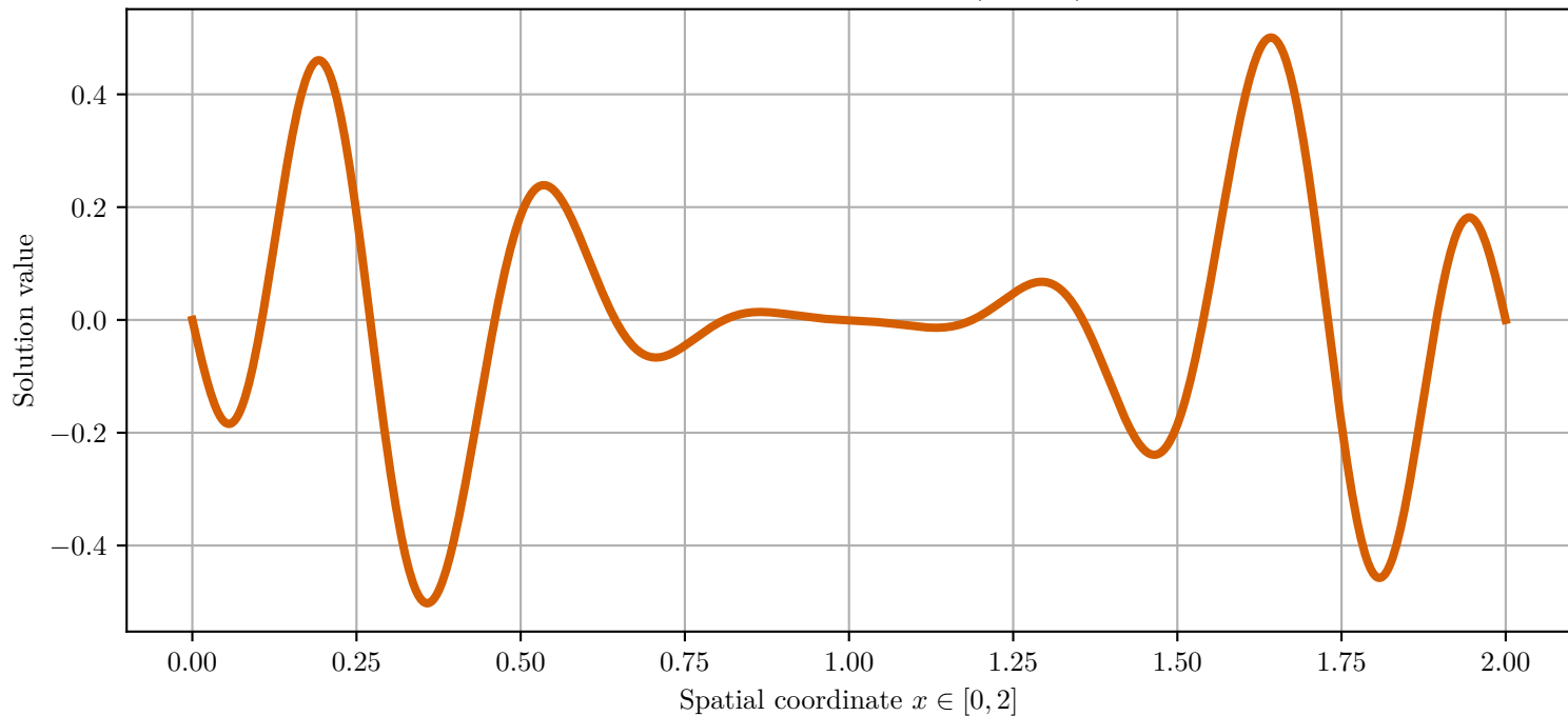
Approximate Solution: u(x, 0.25)
