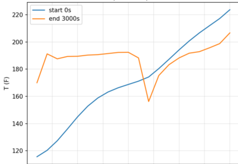
Liquid flow profile
