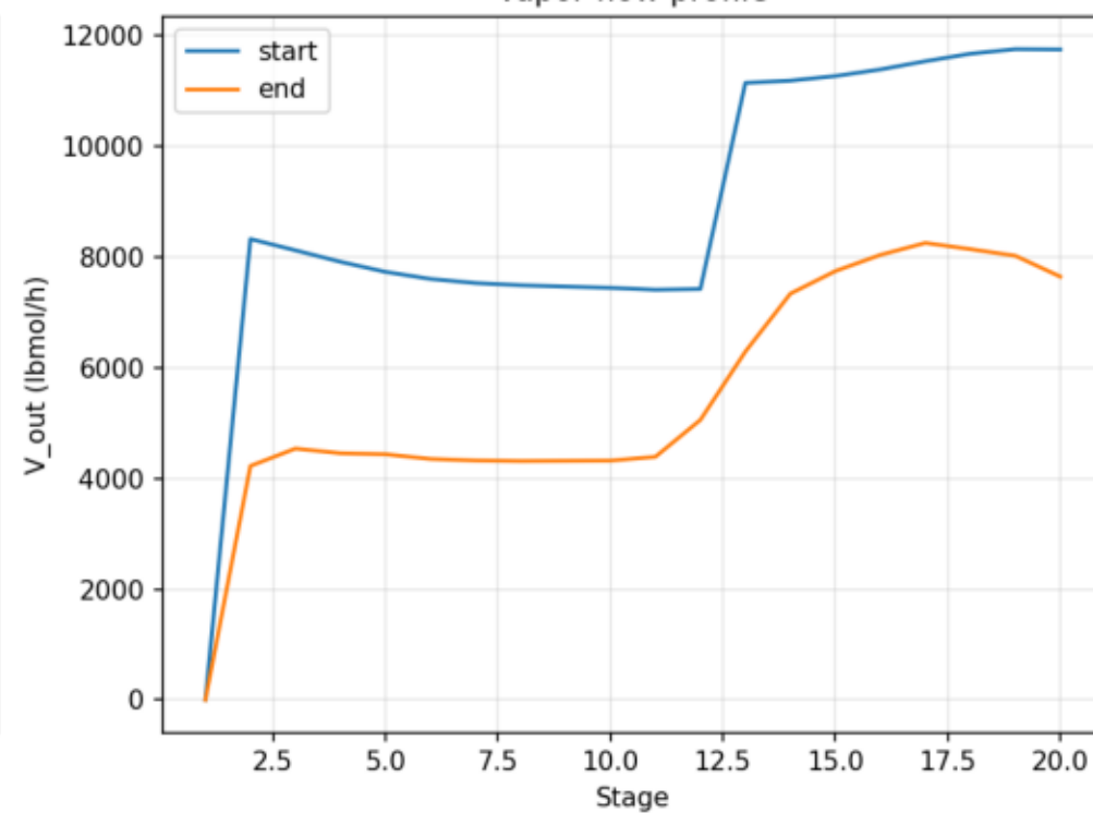
Vapor flow profile
