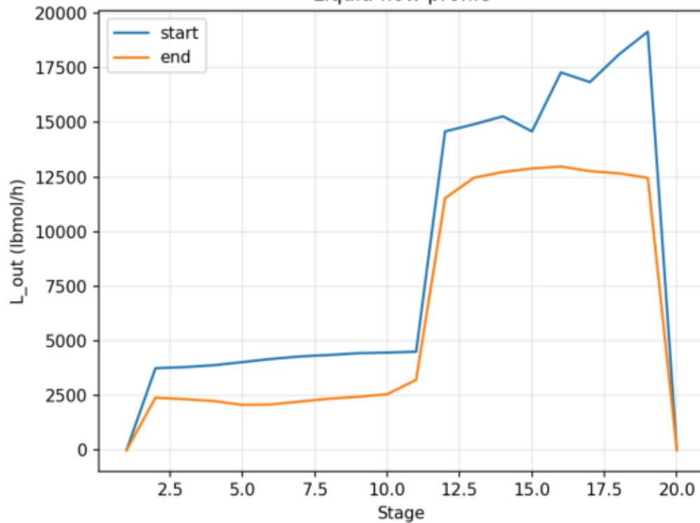
Liquid flow profile
