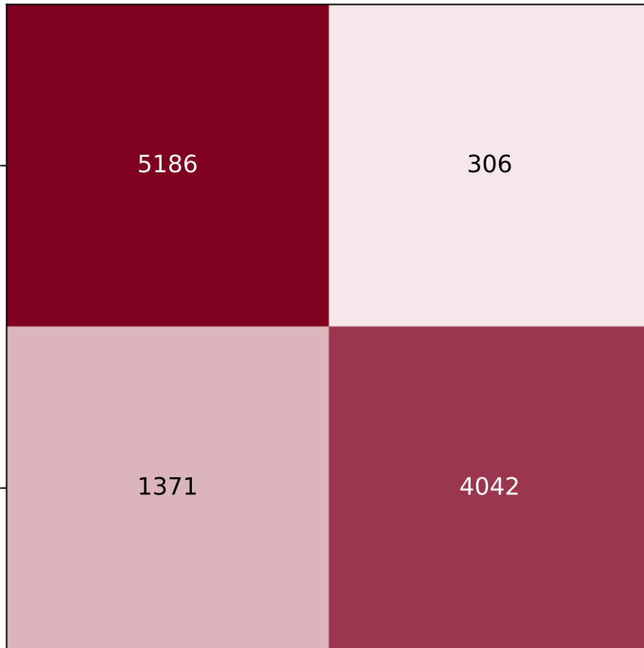
Confusion Matrix - ResNet50
