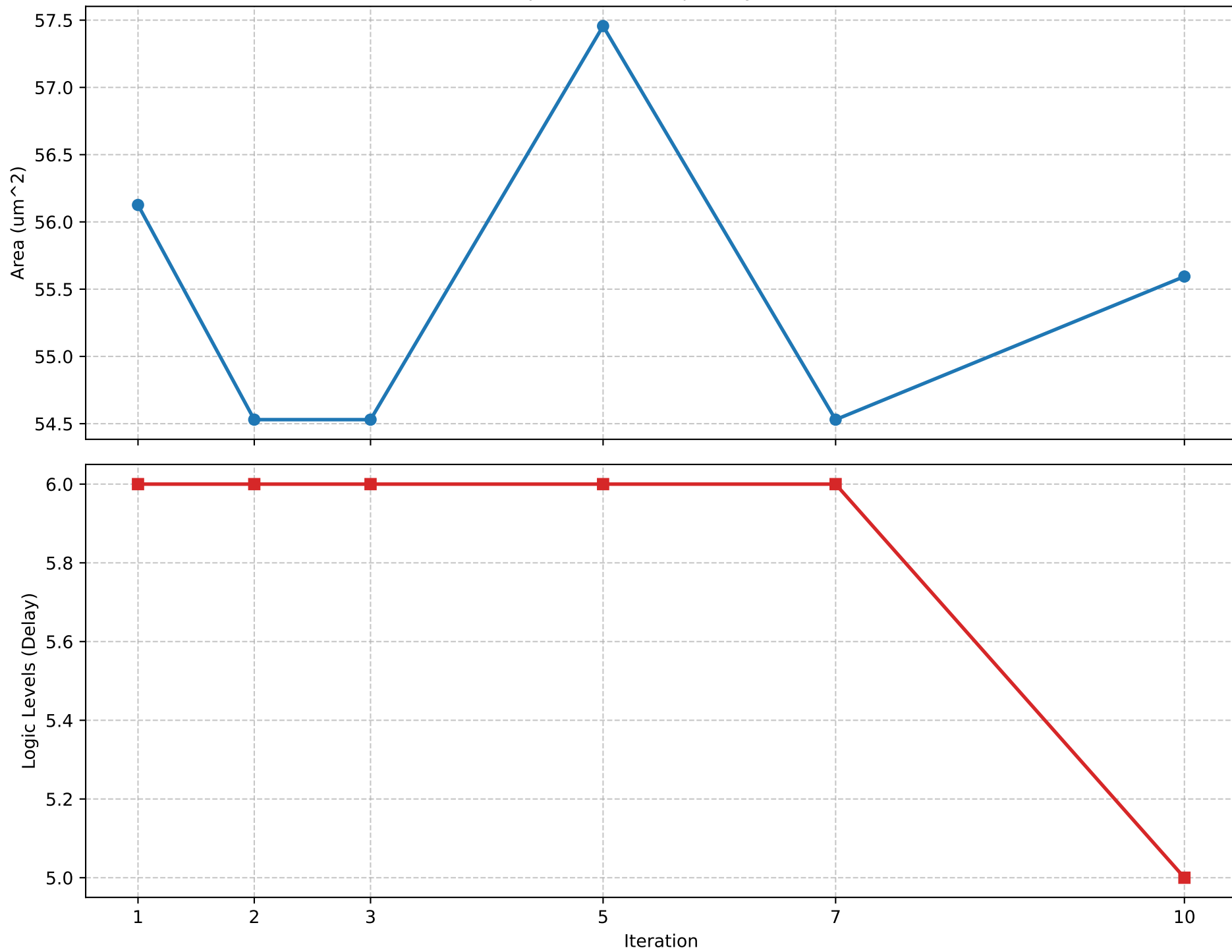
PPA Optimization Trajectory - Mode B
