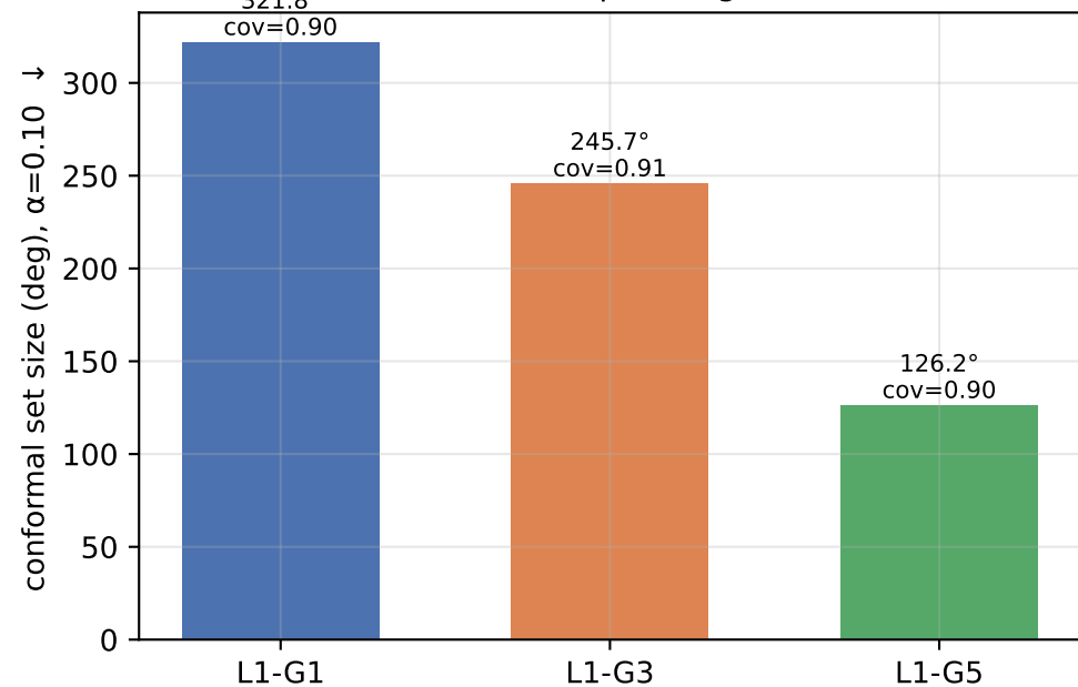
(a) OCS-only conformal set size tightens with geometry (current simulated split, target cov=0.90)
